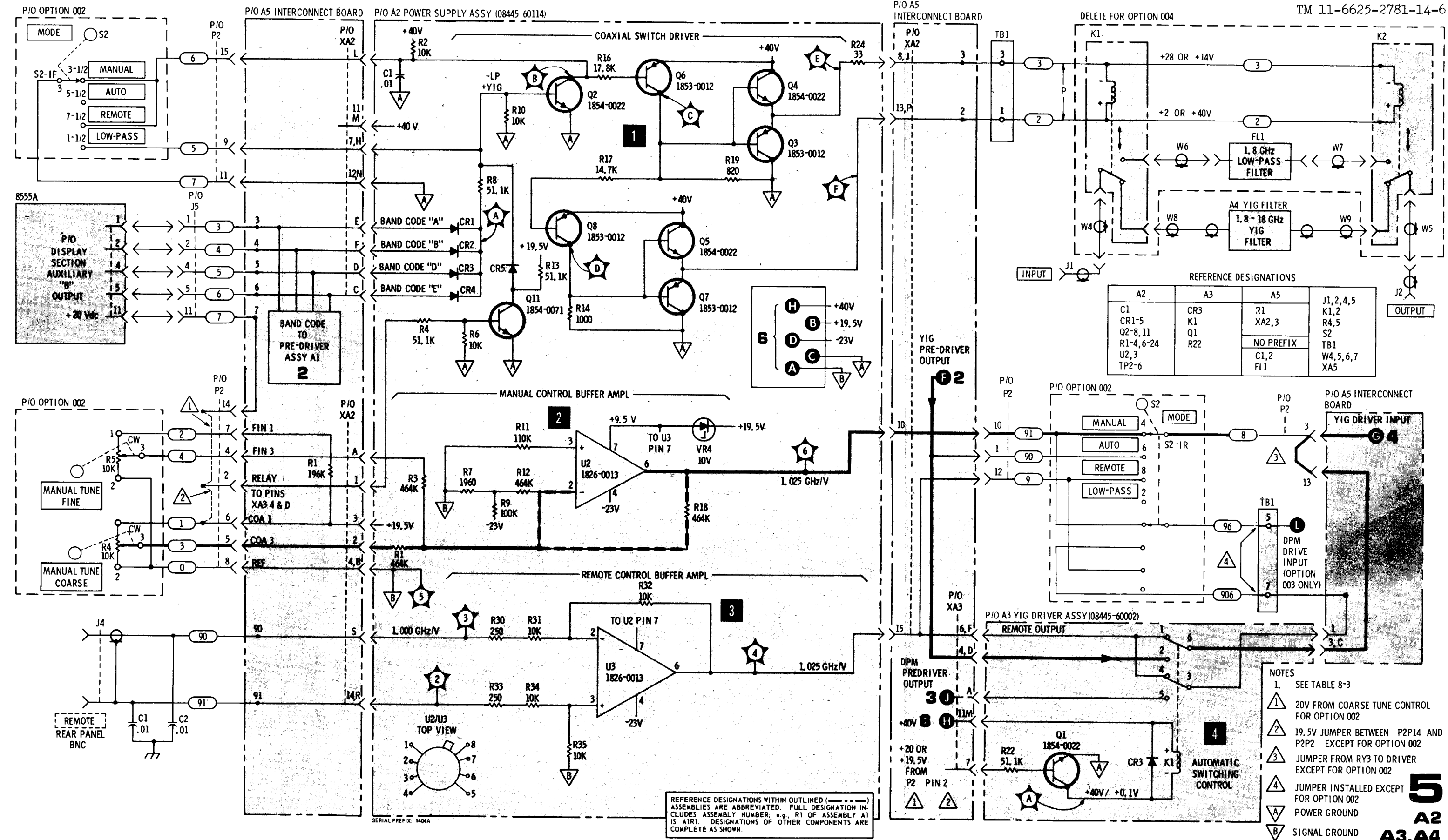
Figure 8-19. Remote and Manual Control Amplifiers/Switching Circuit Schematic Diagram
