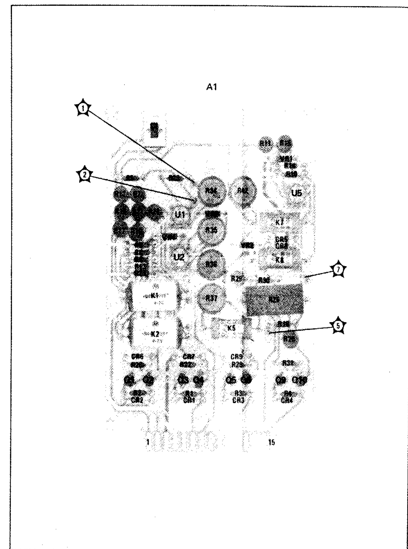
Figure 8-9. A1 Predriver Assembly of 8445B (Except Option 003)
