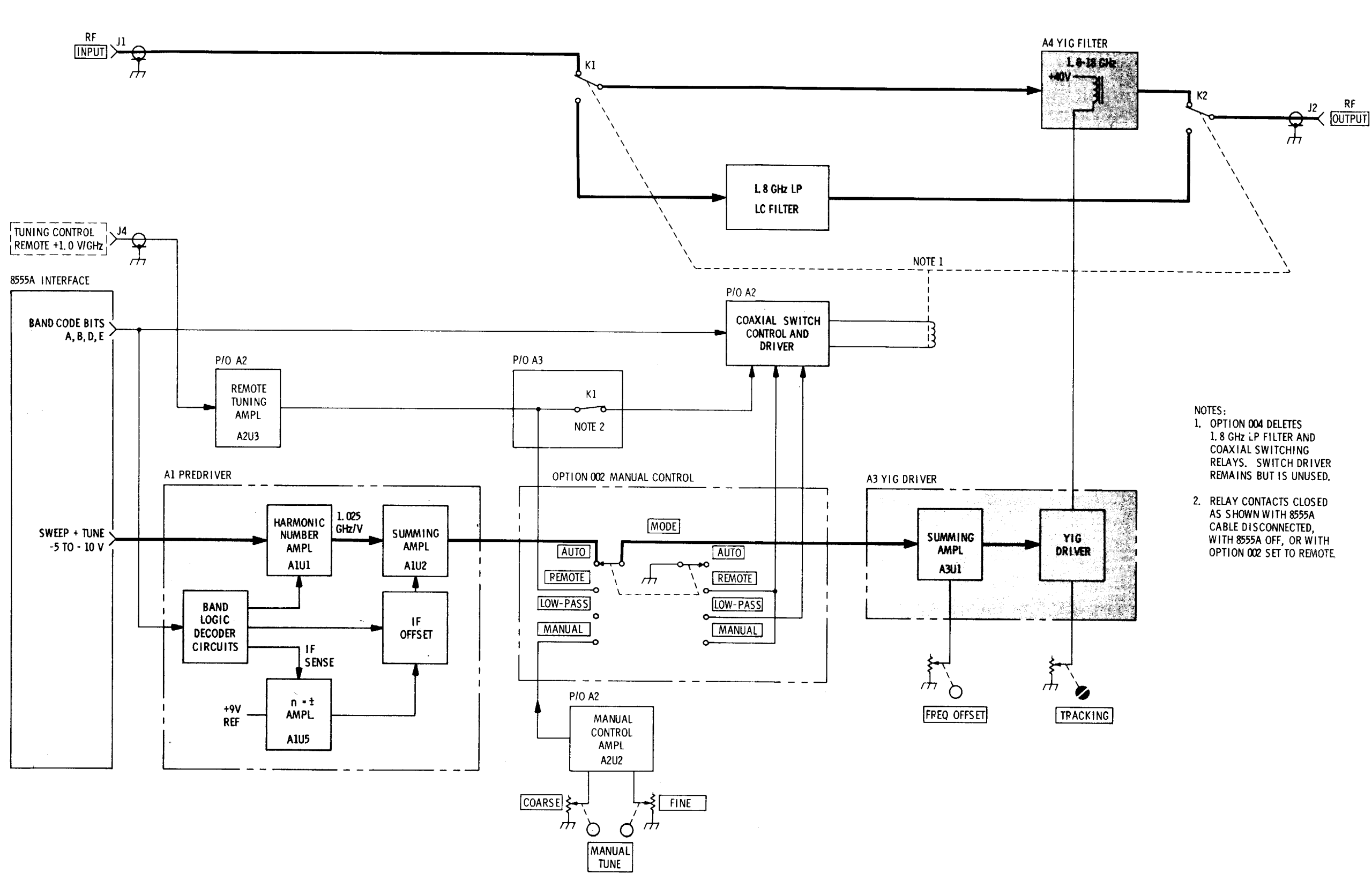
Figure 8-6. Block Diagram of 8445B With Option 002 Circuits Unshaded
