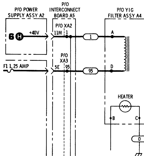
Figure 7-2. Partial Schematic correction for Service Sheet 4. (P/O CHANGE C)
