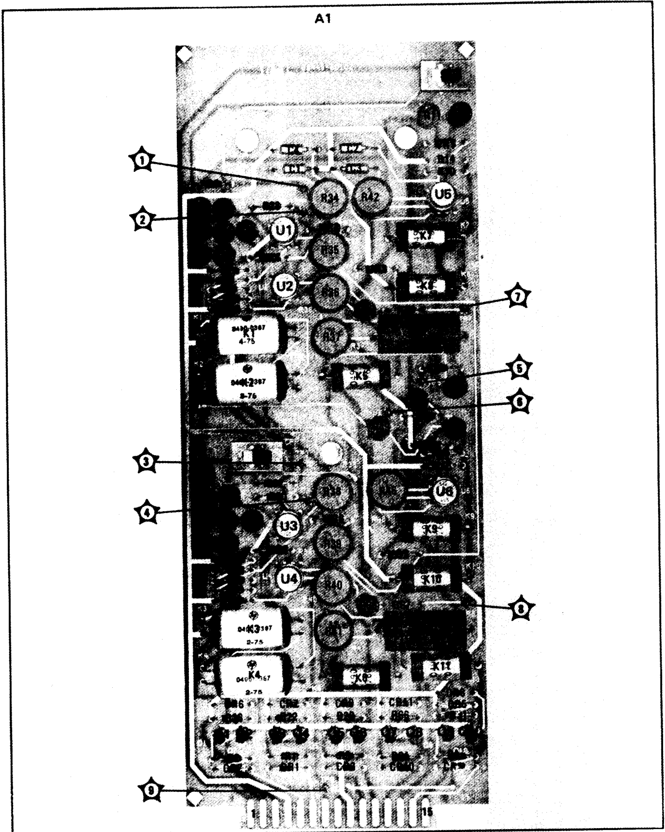
Figure 8-13A. A1 Predriver Assembly of 8445B (Option 003) (Change 1)
