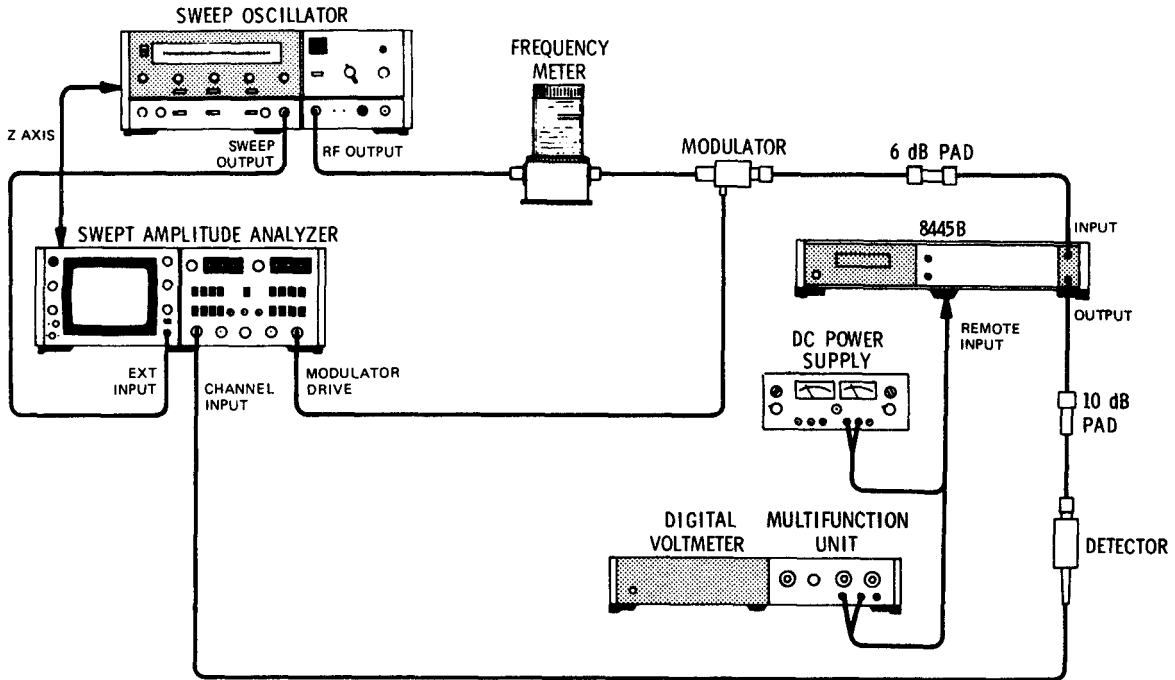
Figure 5-3. YIG Driver Adjustment Test Setup
