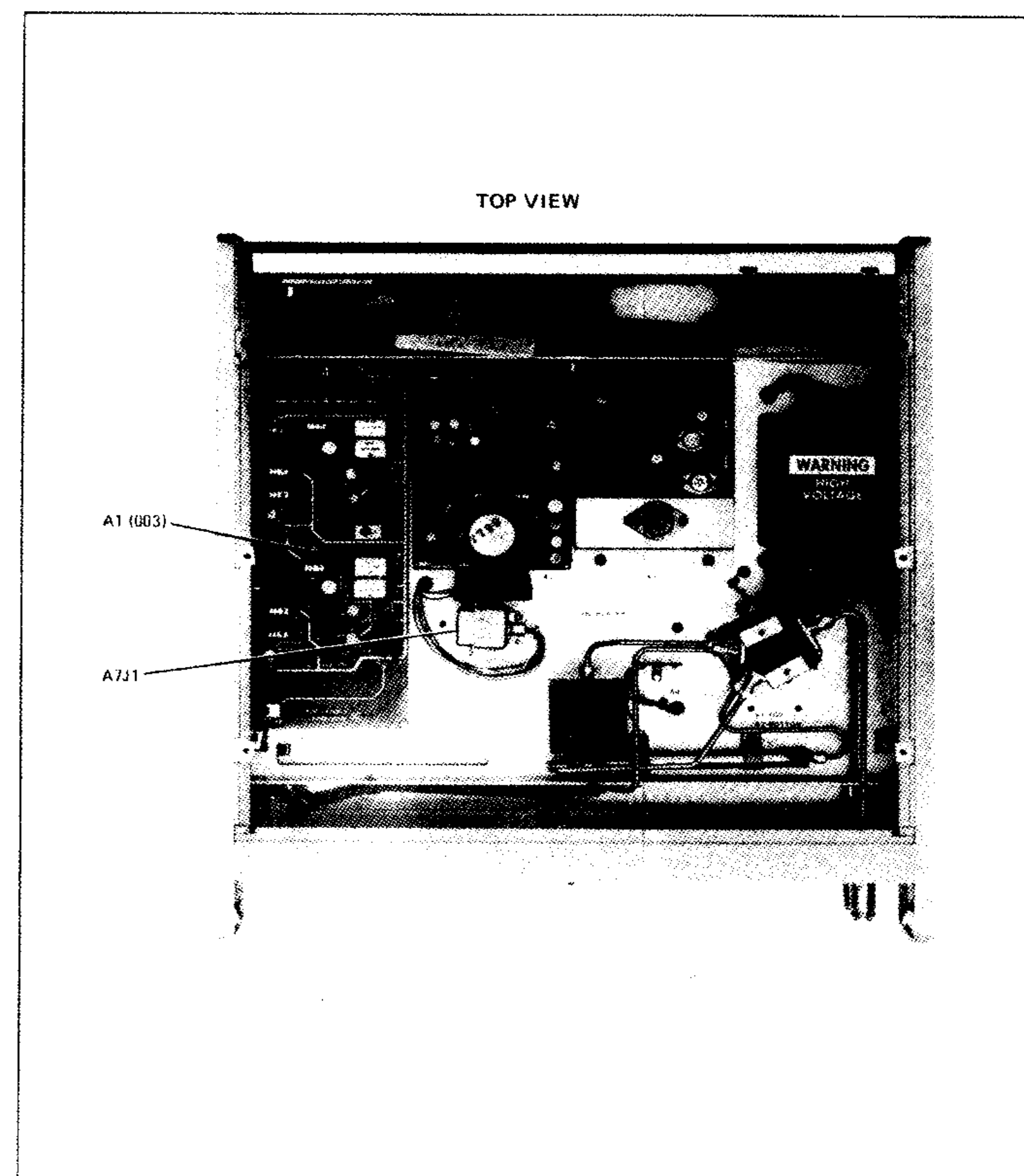
Figure 8-12. Top View of 8445B, Option 003 With A7 Removed.
