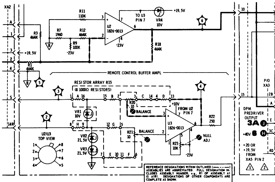
Figure 7-3. Partial schematic correction for Service Sheet 5. (P/O CHANGE C)
