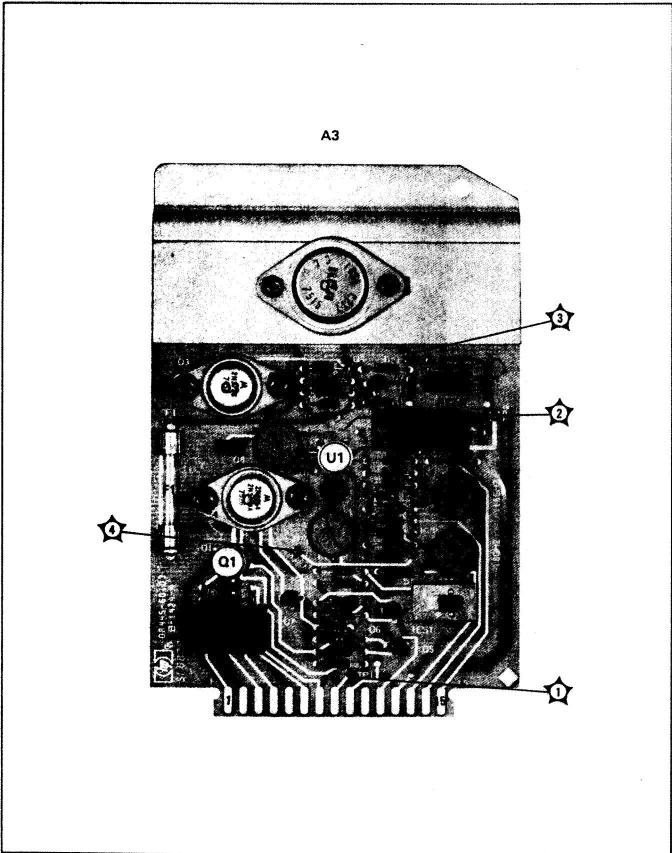
Figure 8-16A. A3 YIG Driver Assembly (Change 1)
