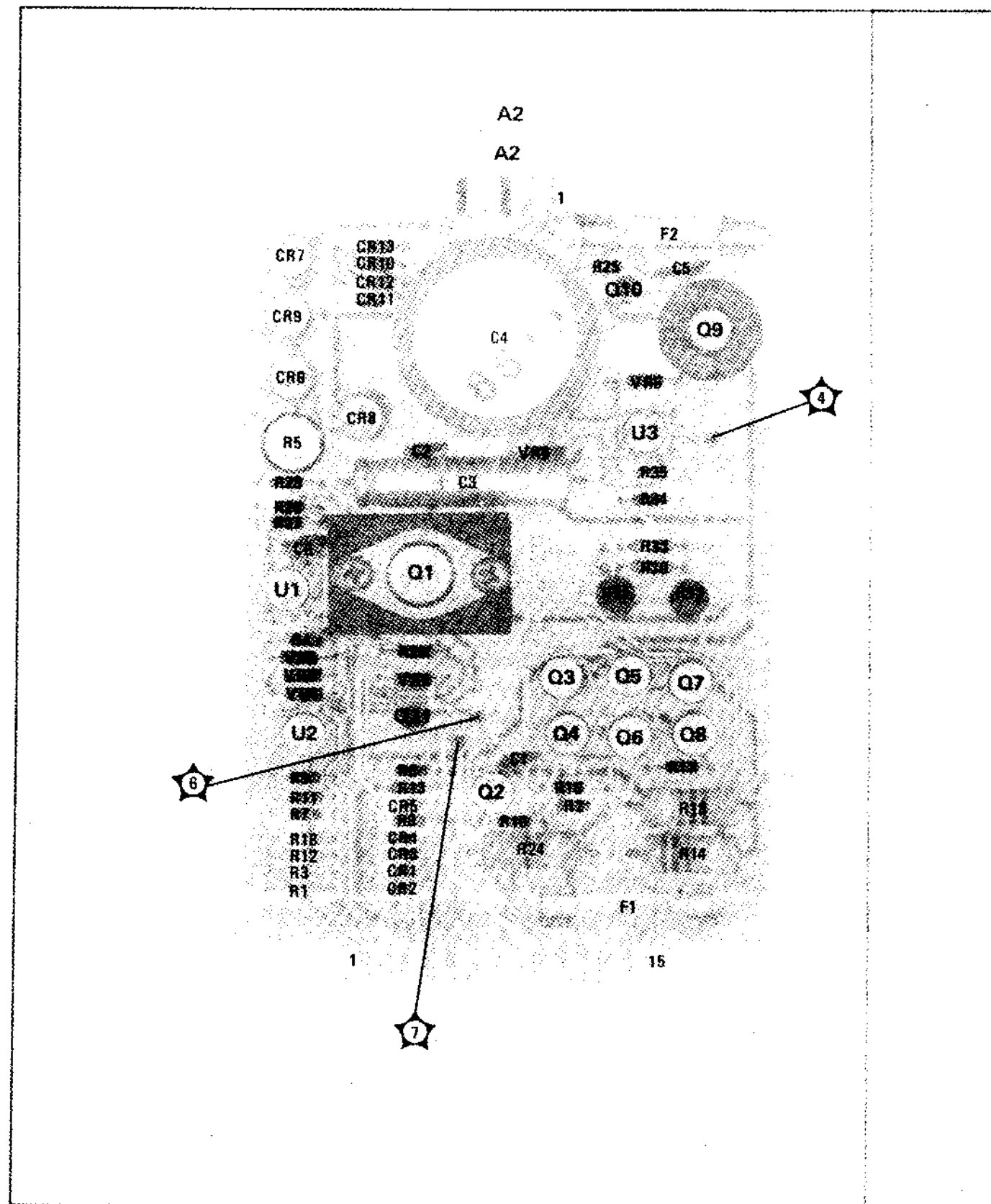
Figure 8-20. A2 Power Supply and Filter Switching Assembly
