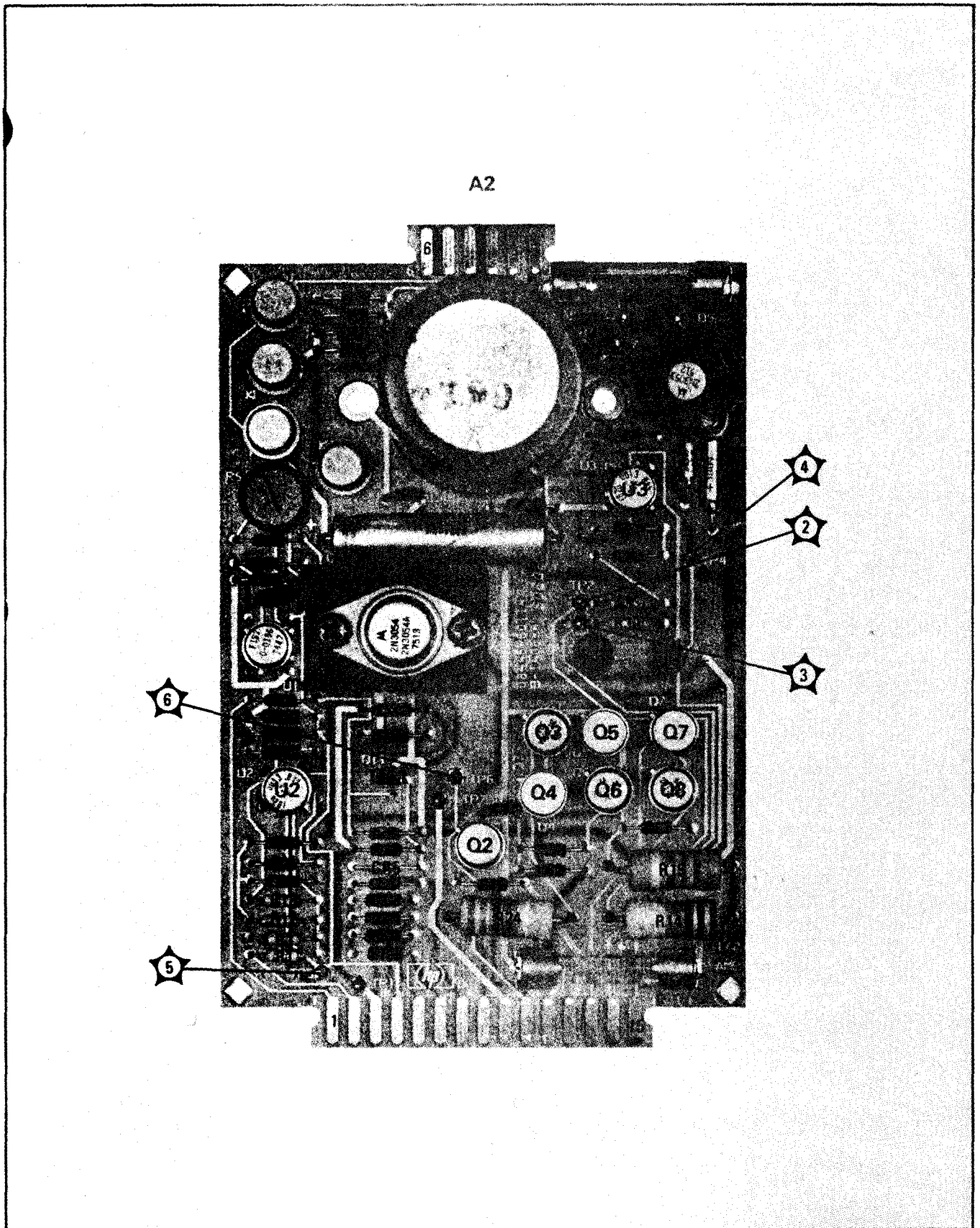
Figure 8-18A. A2 Power Supply Assembly, Remote and Manual Control Amplifiers/Switching Circuit (Change 1)
