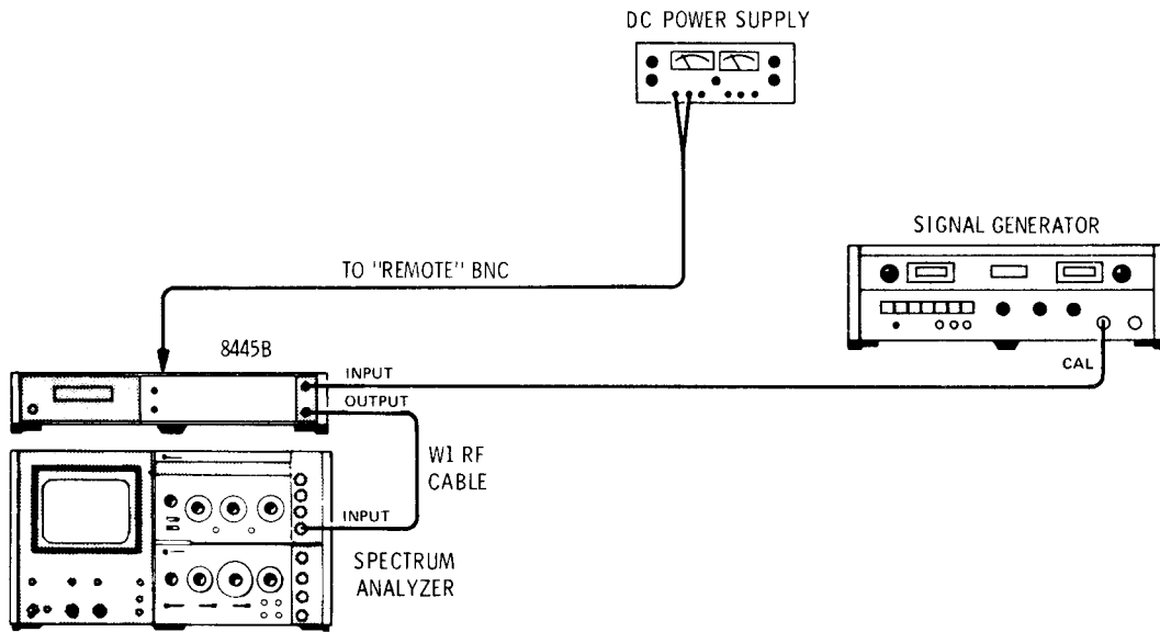
Figure 4-1. Out-of-Band Rejection Test Setup
