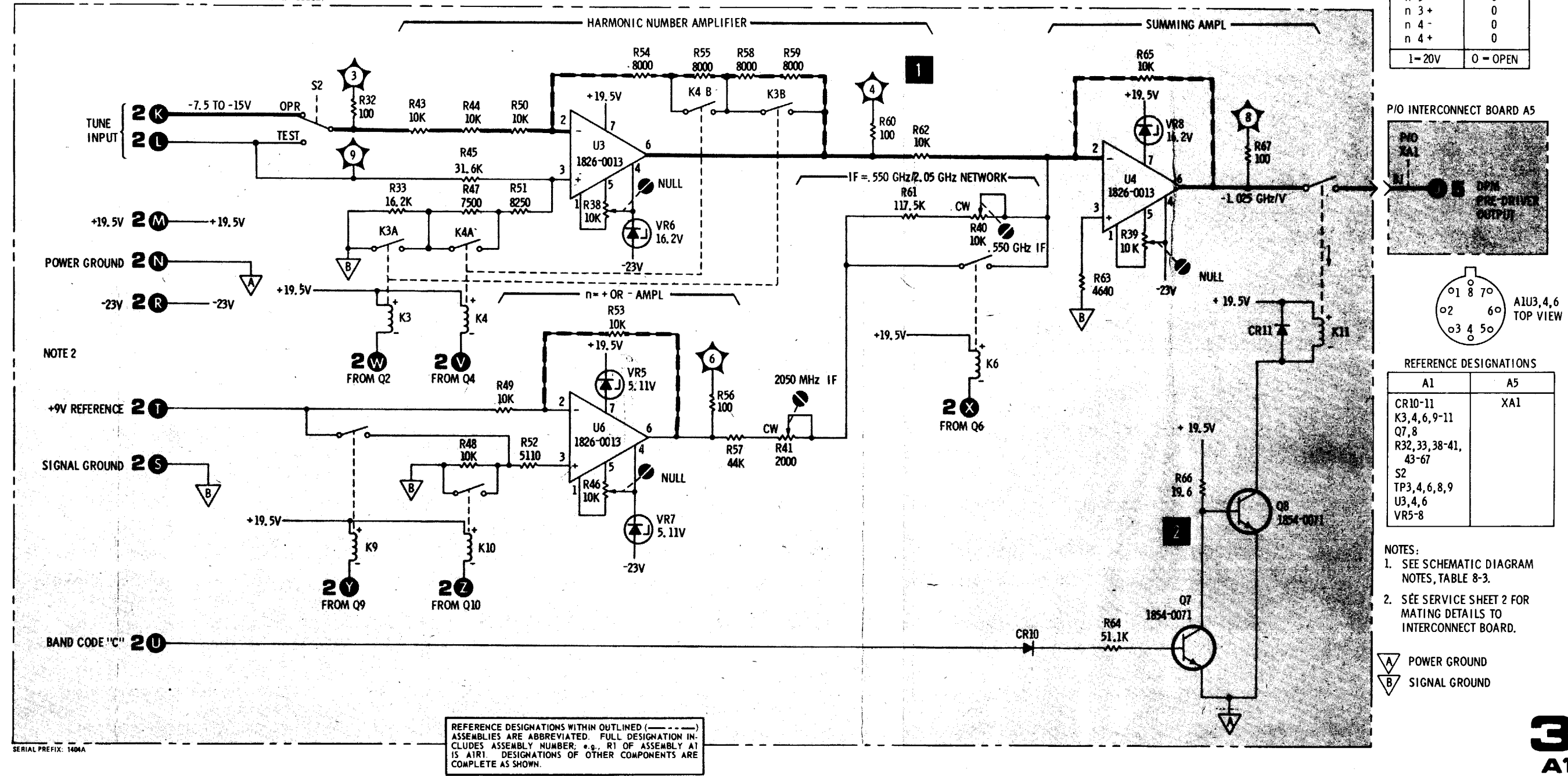
Figure 8-15. DPM Pre-driver Schematic Diagram
