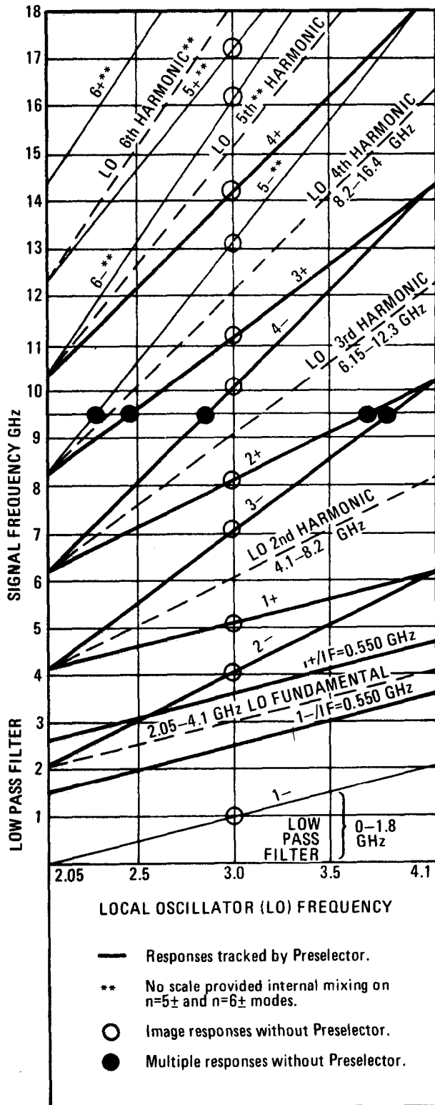
Figure 3-1. Spectrum Analyzer Tuning Curves and Responses
