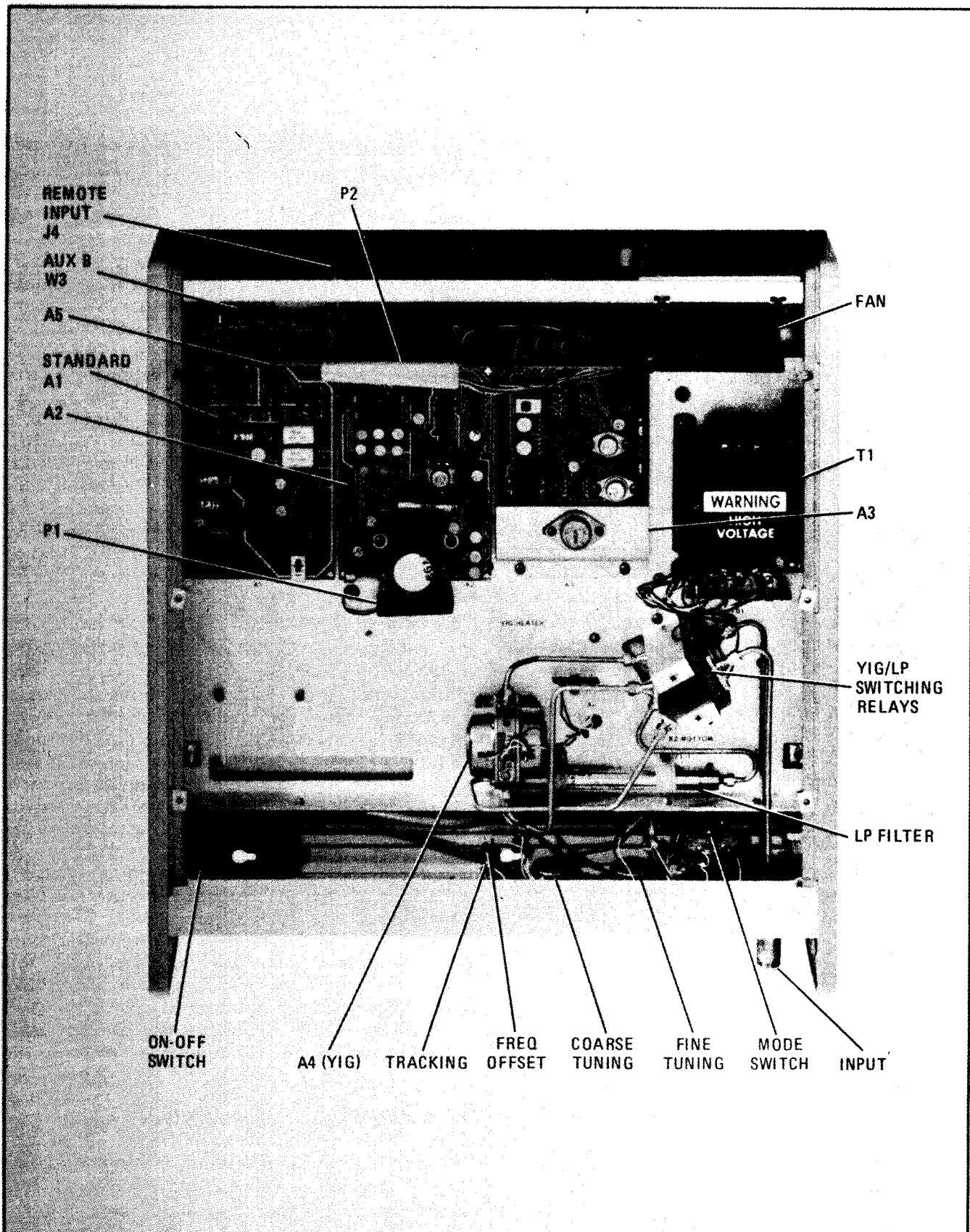
Figure 8-4. Top View of 8445B With Option 002 Panel Switches and Controls
