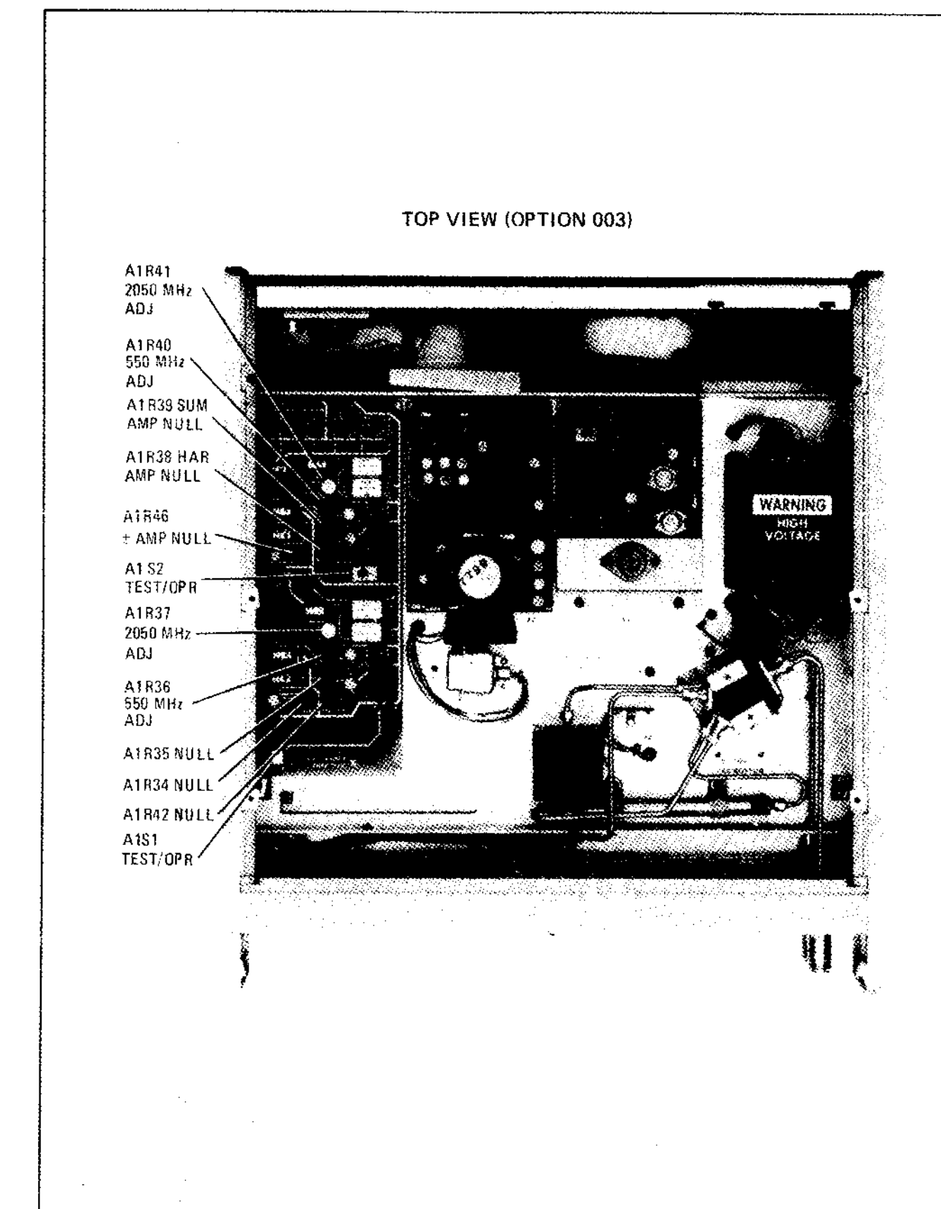
Figure 8-23. Option 003 A1 Adjustment Controls
