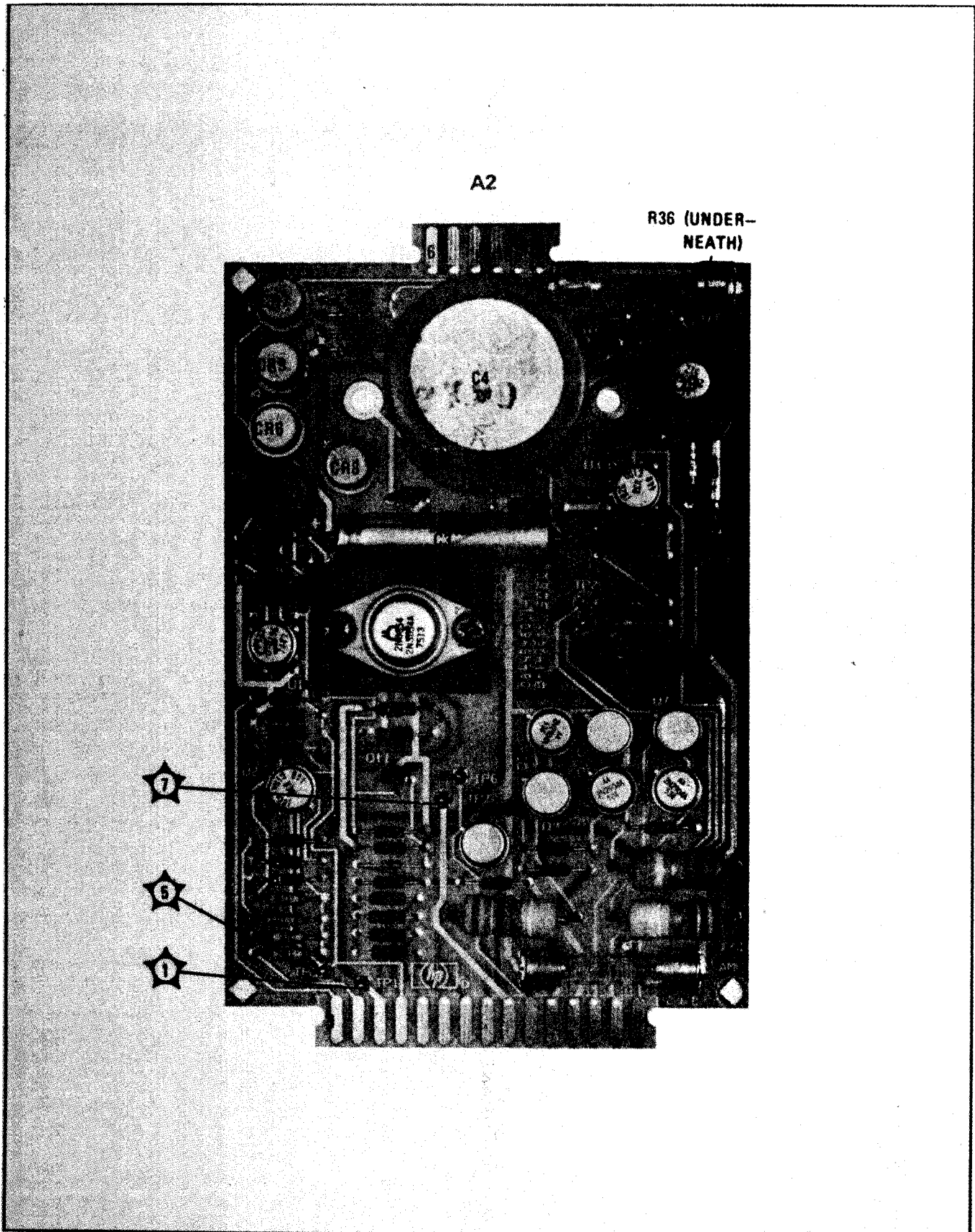
Figure 8-20A. A2 Power Supply Assembly, Supply Voltage Circuits (Change 1)
