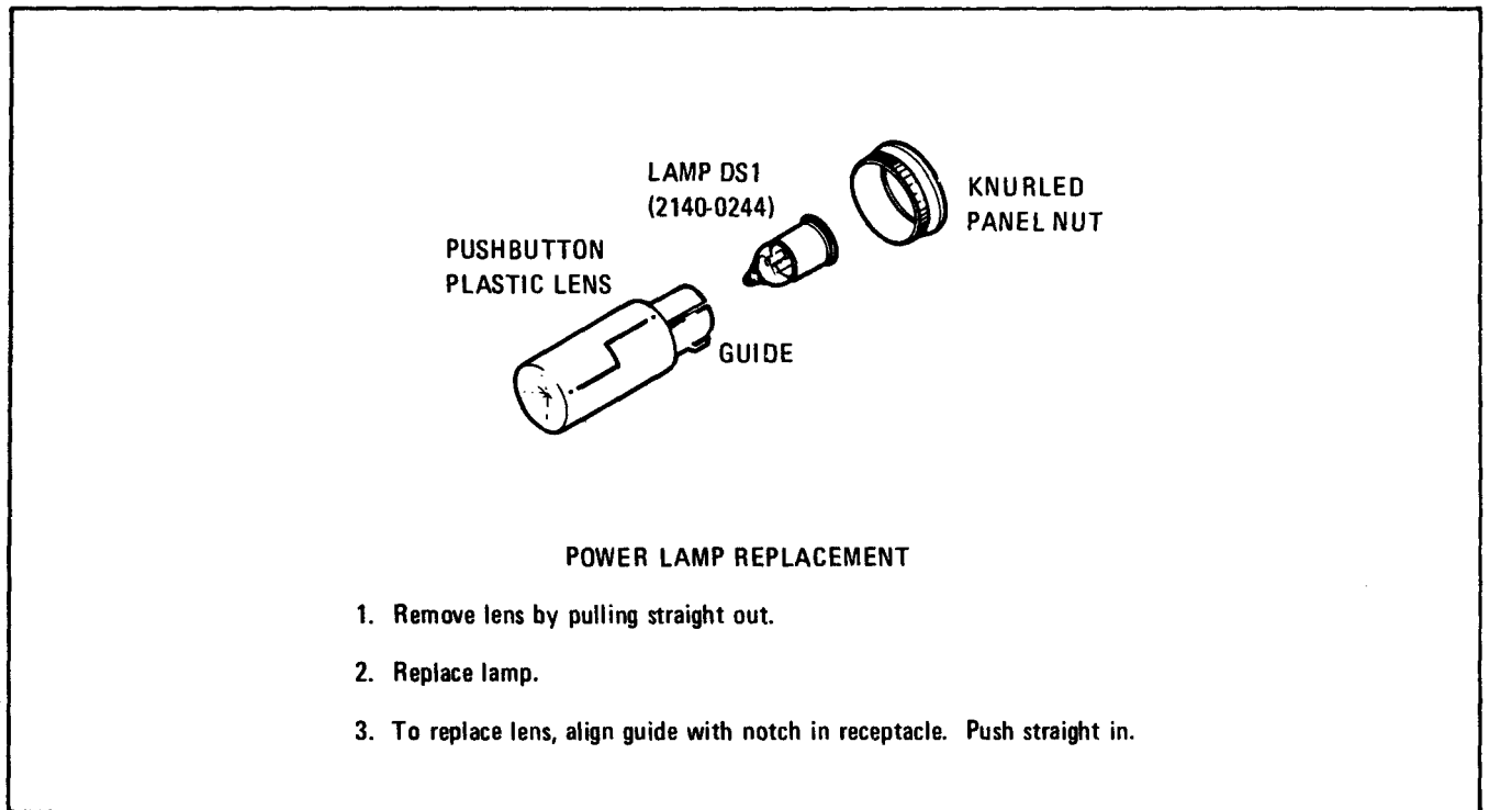
Figure 3-6. Power Lamp Replacement
