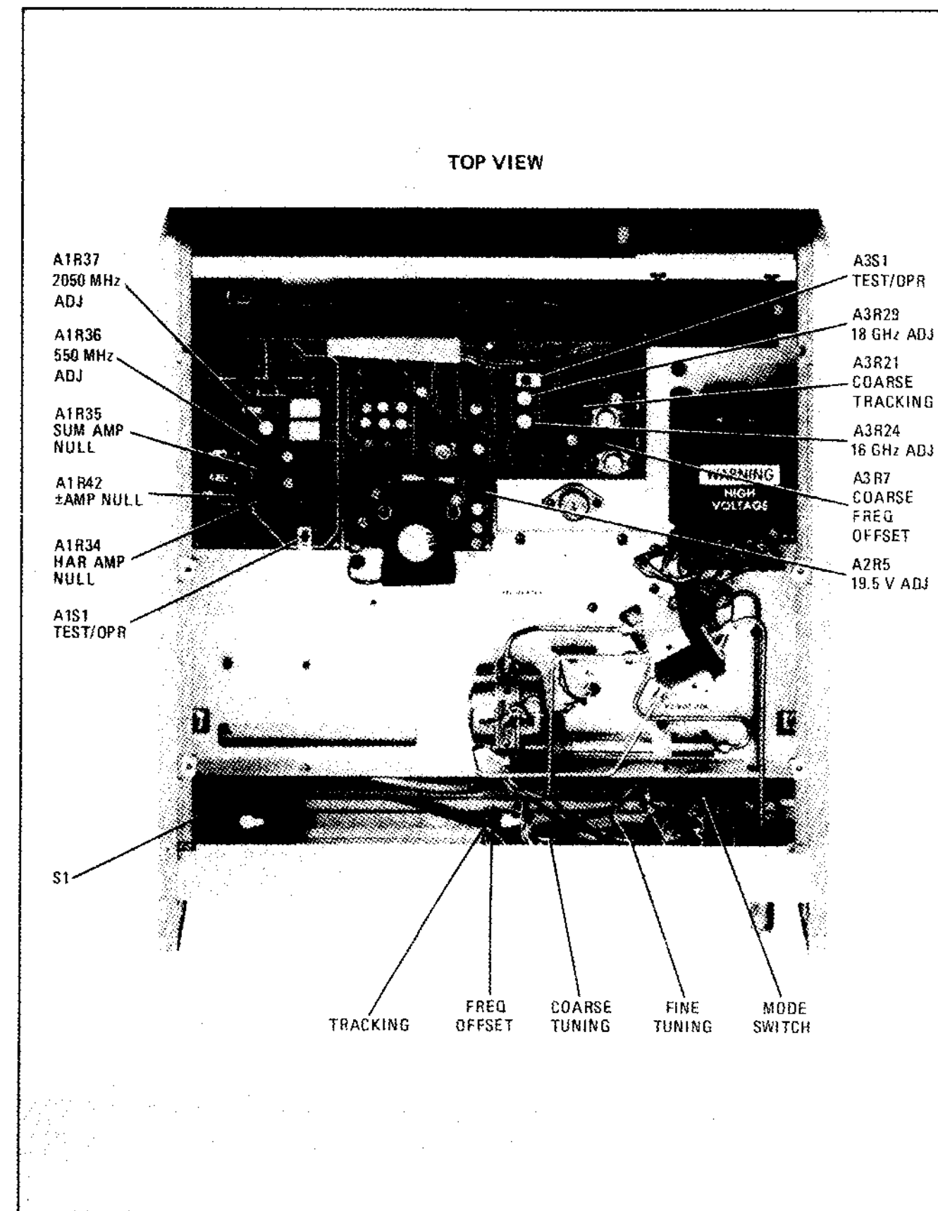
Figure 8-22. Adjustment Controls
