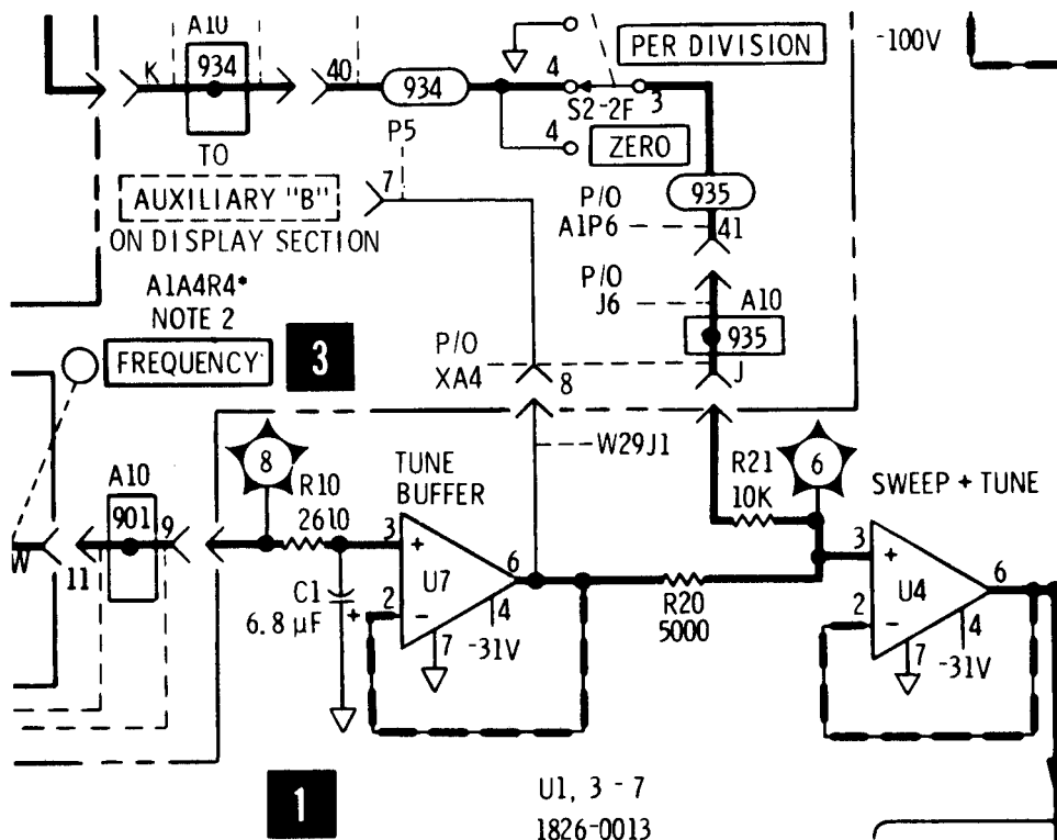
Figure B-3. Partial Schematic of Modified A4 Assembly
