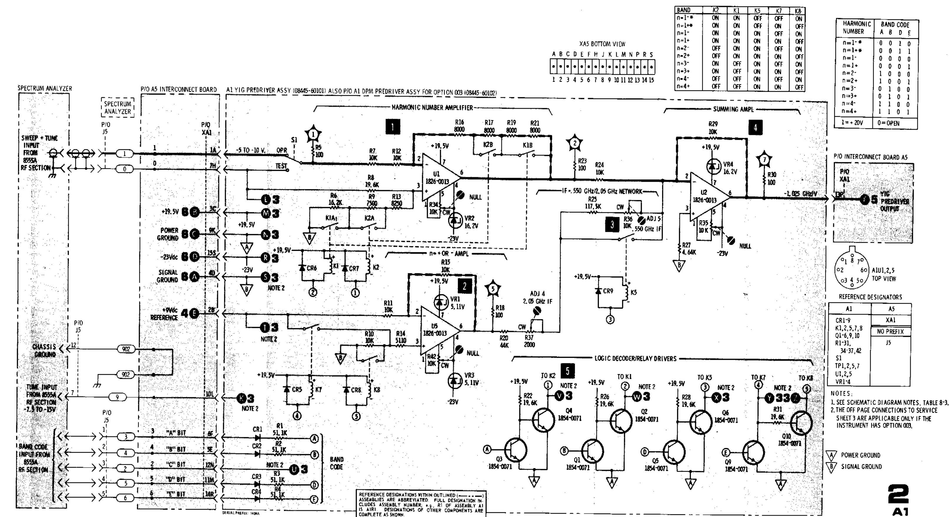
Figure 8-10. YIG Predriver Schematic Diagram
