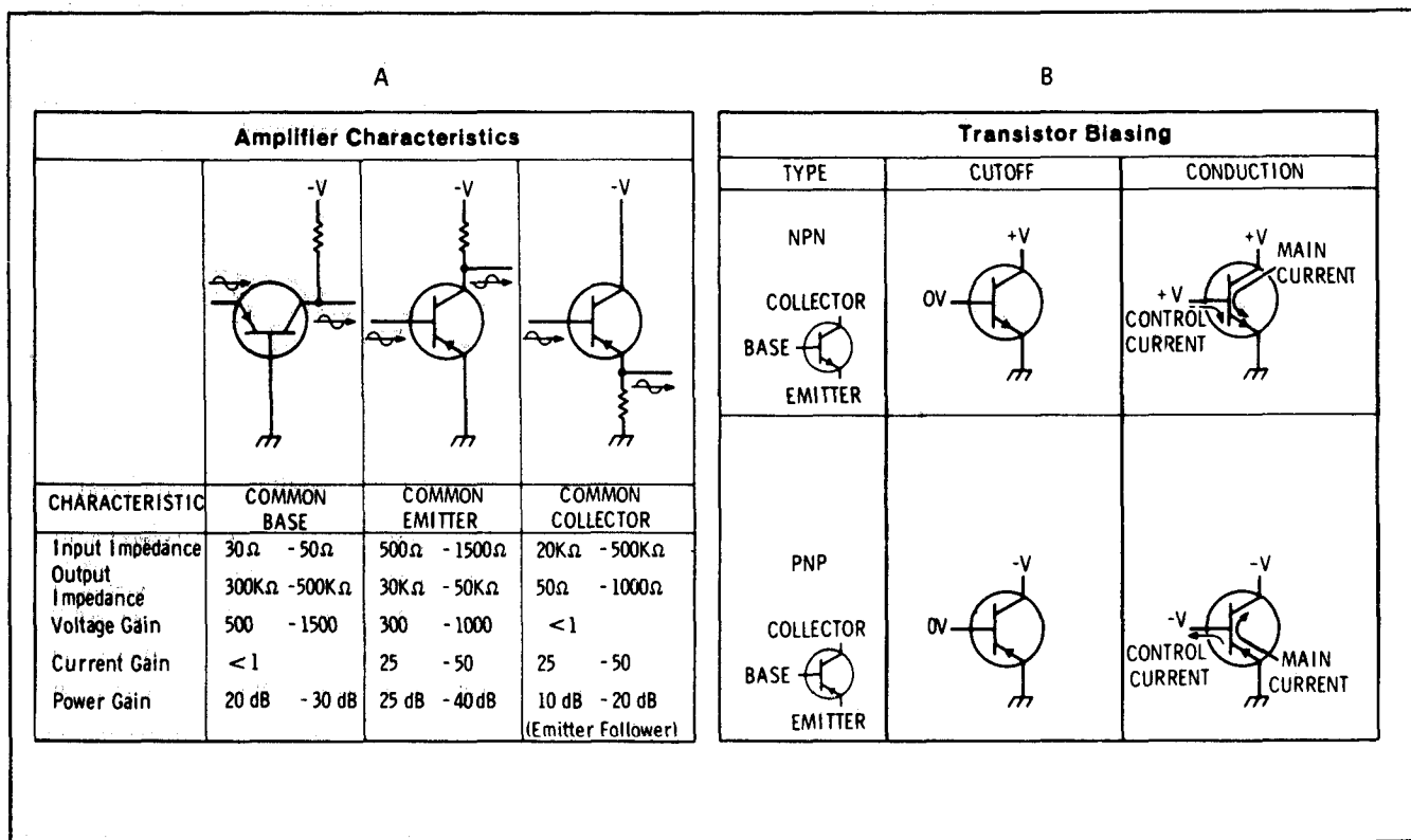
Figure 8-1. Transistor Characteristics and Biasing.
