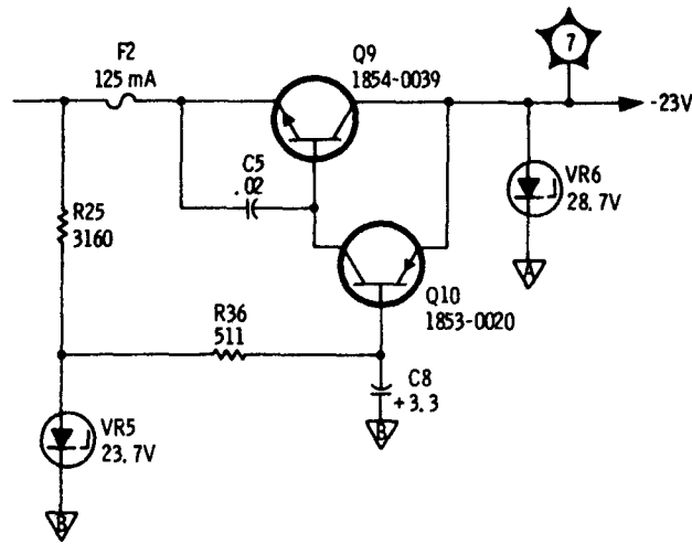
Figure 1. Partial Schematic of Figure 8-10(P/O Change 1)
