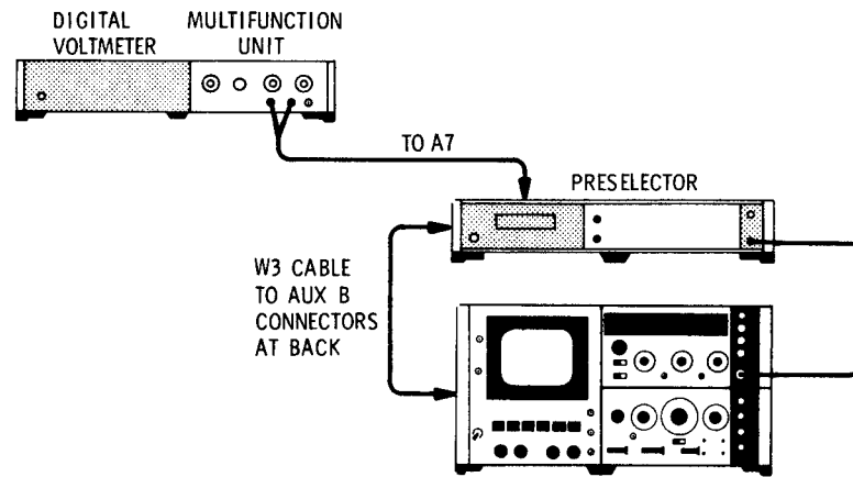
Figure 5-4. Digital Panel Meter Adjustment Test Setup.
