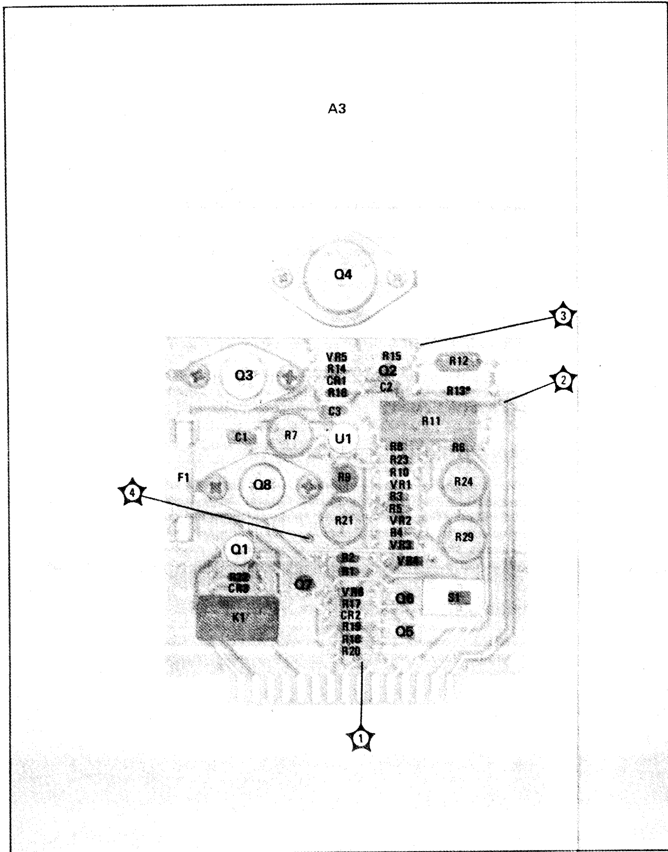
Figure 8-16. A3 YIG Driver Assembly
