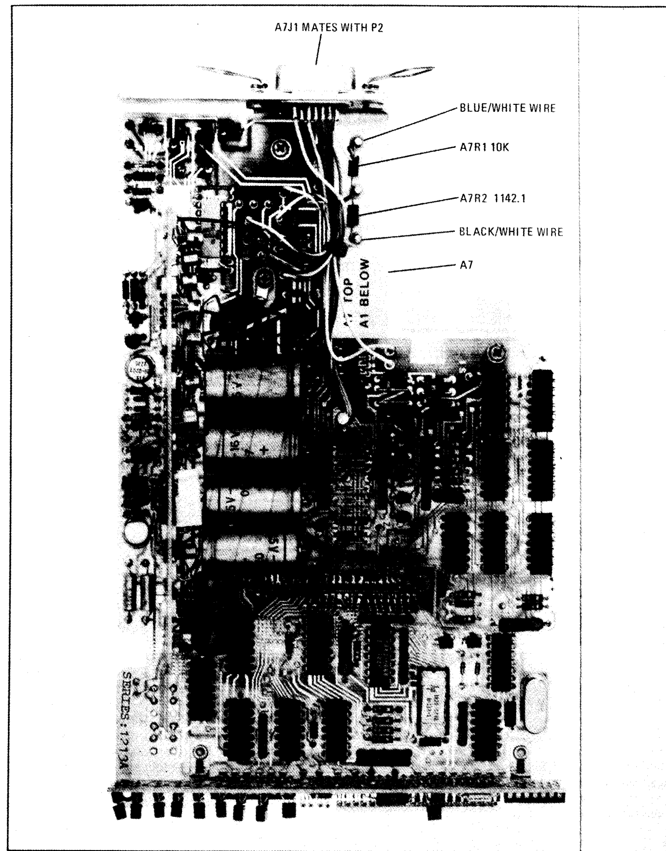
Figure 8-14. A7 Display Board (See Option 003 Supplement For Details) A7 8445B.
