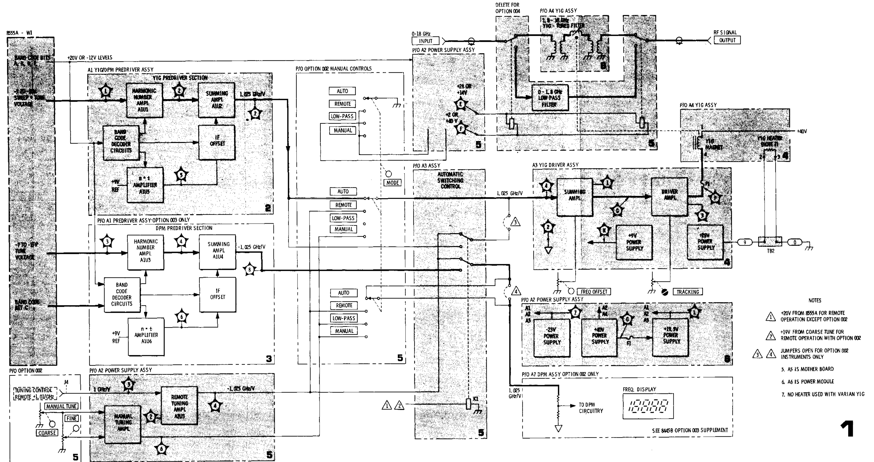
Figure 8-8. Comprehensive Block Diagram Including Options 002 and 003
